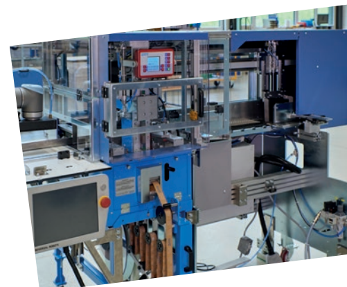
Banding Unit
